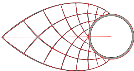
Figure 10: Pattern constructed according to the Michell's Theorem for optimal material placement. In the cantilever above, the loading is downward at the point with support connections at the ring. The geometric patterning eliminates bending from the members and resolves forces to 'pure' tension and compression. If the diagram were to be of higher accuracy, the members would be straight lines.
